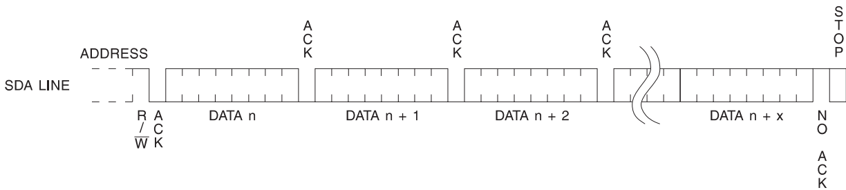
Figure 4. Sequential Read
