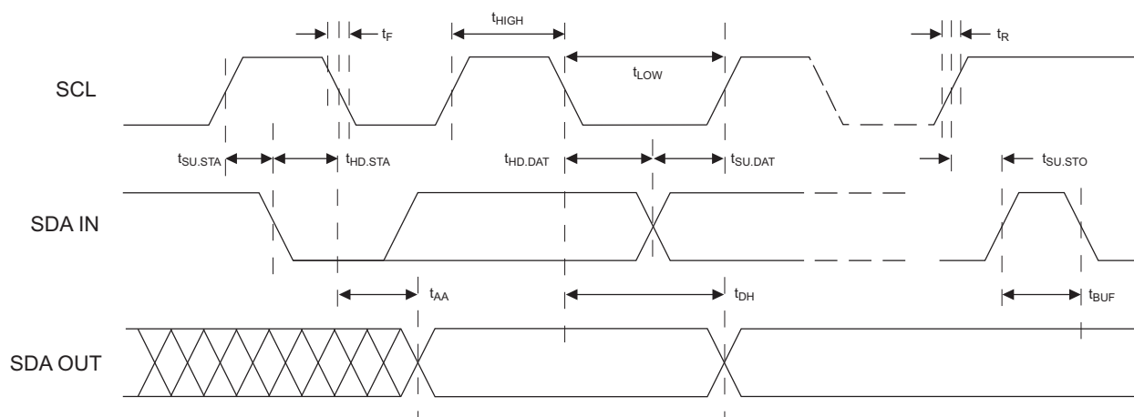
Figure 8-1. Bus Timing
