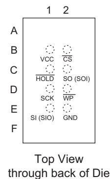
Figure 2-3. 8-ball dBGA (WLSCP)
