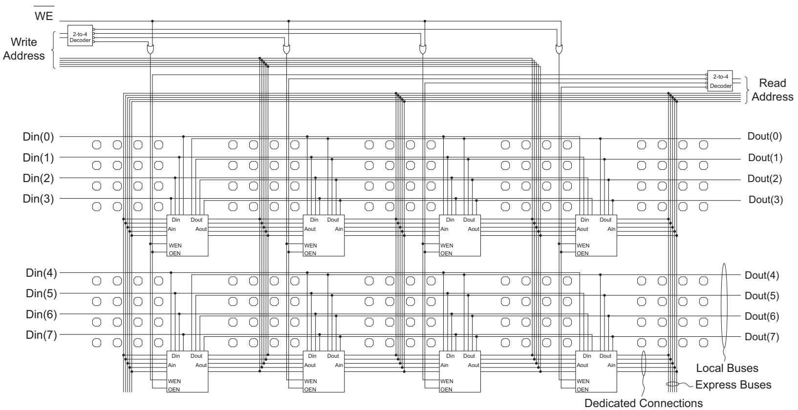
Figure 6-3. RAM Example: 128 x 8 Dual-ported RAM (Asynchronous)
