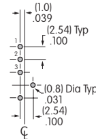
V Terminals
