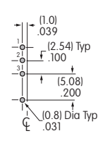
V1 Terminals
