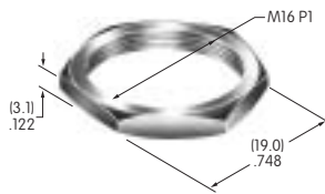
AT056 Dress Cap Nut Chrome/brass Series: M P S
