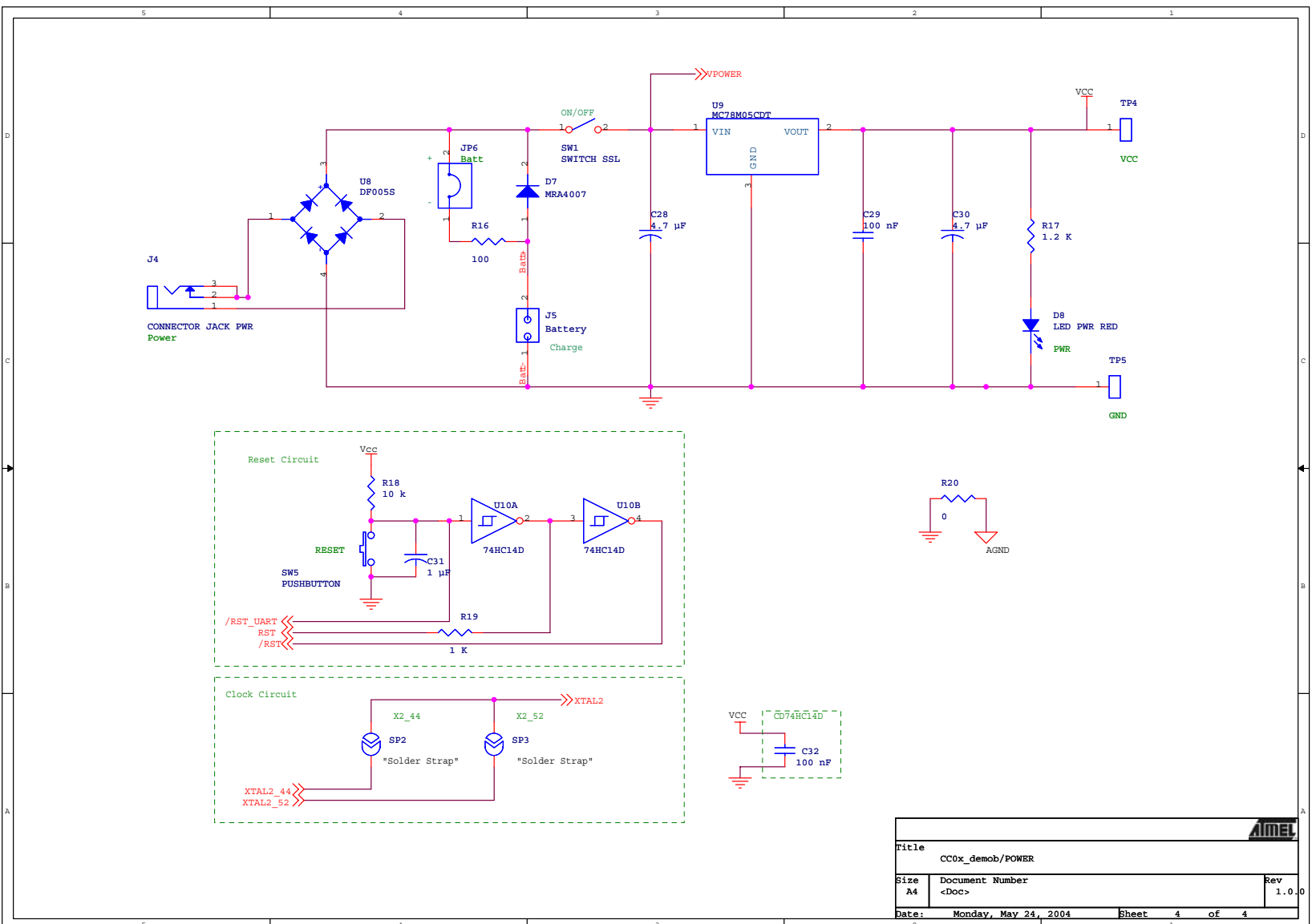
Figure 4-6. AT89STK-06 Board Schematics (4 of 4)
