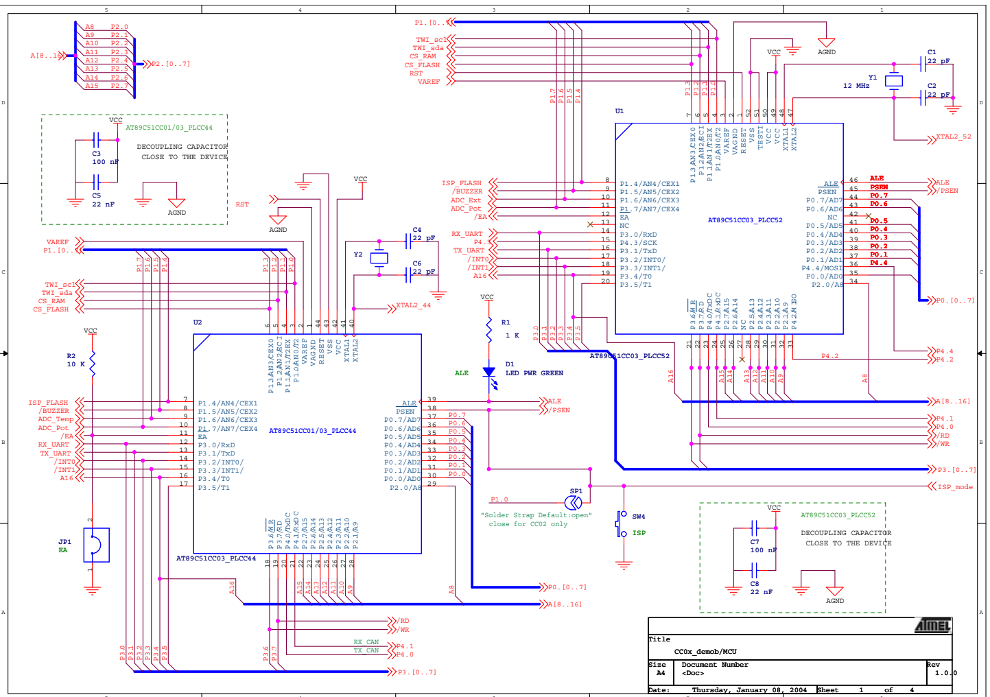
Figure 4-3. AT89STK-06 Board Schematics (1 of 4)
