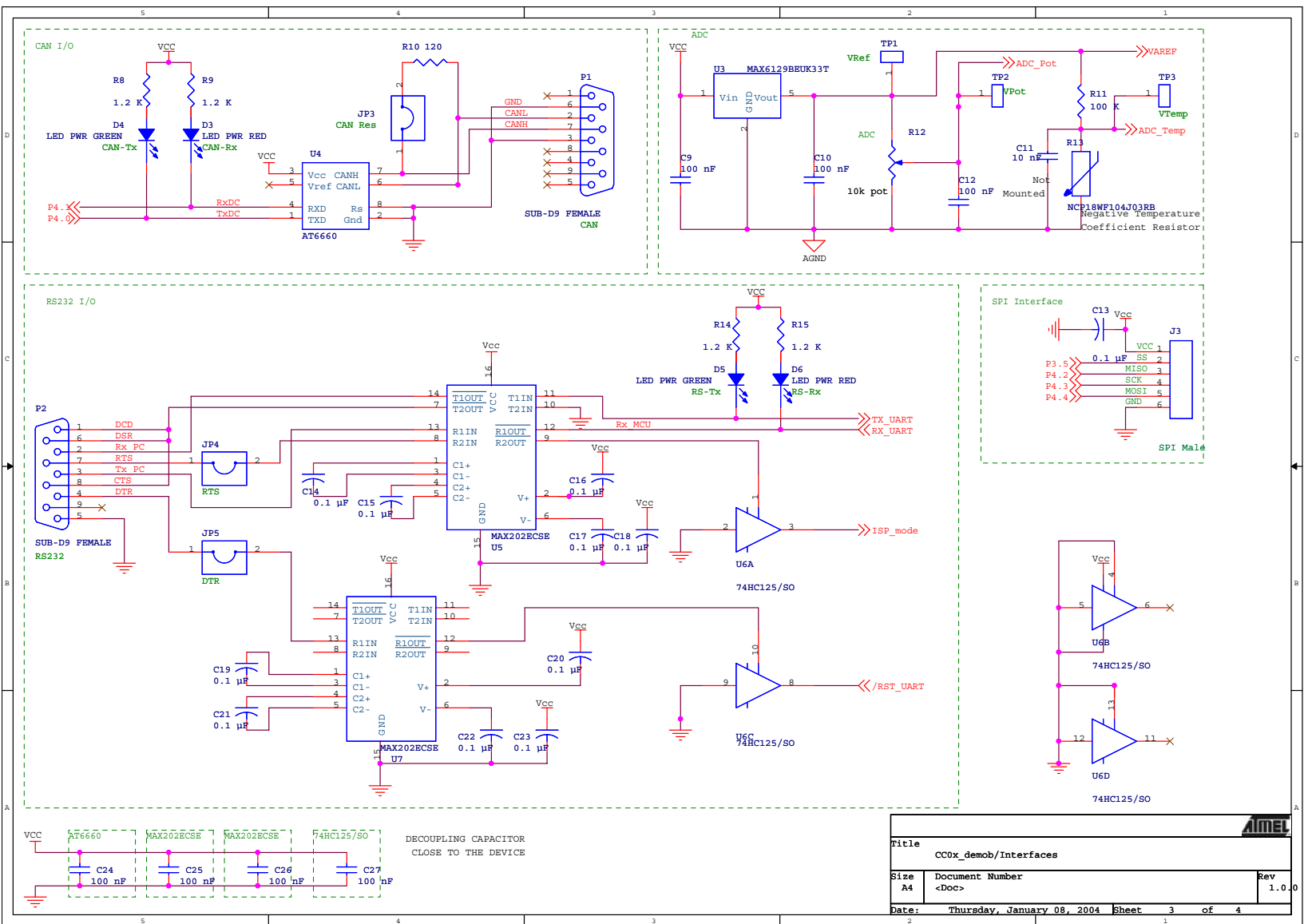
Figure 4-5. AT89STK-06 Board Schematics (3 of 4)
