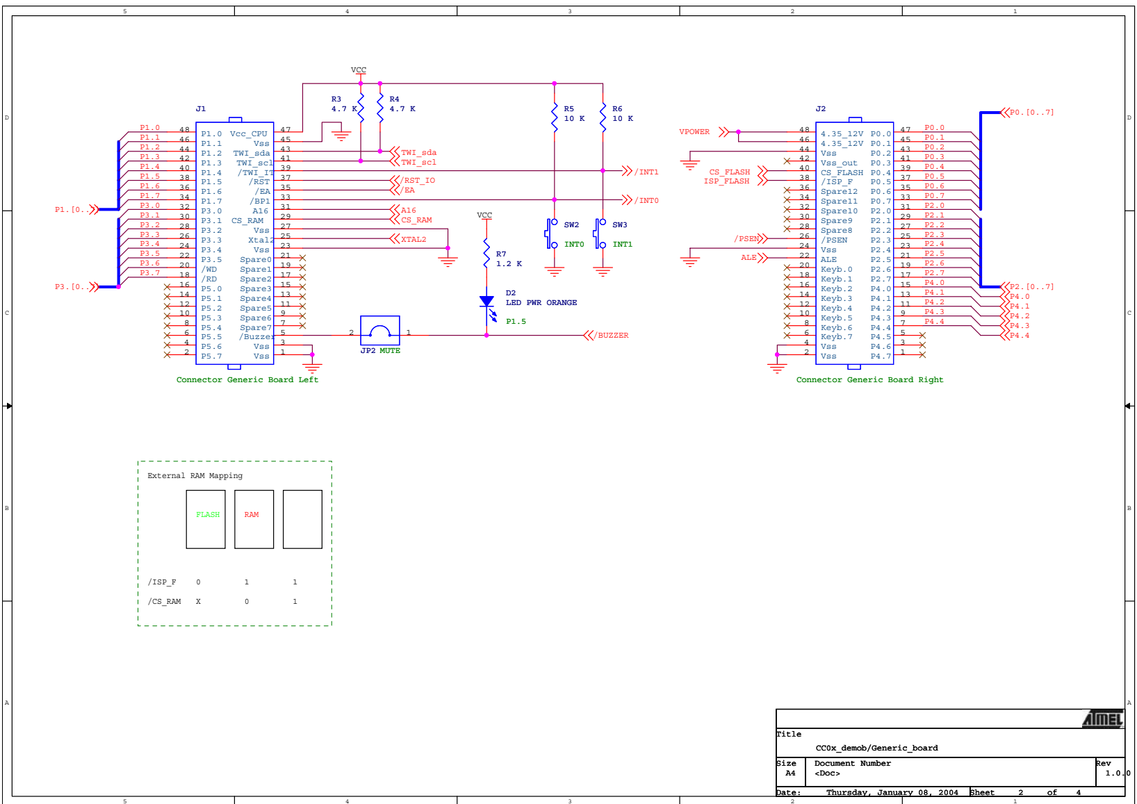
Figure 4-4. AT89STK-06 Board Schematics (2 of 4)
