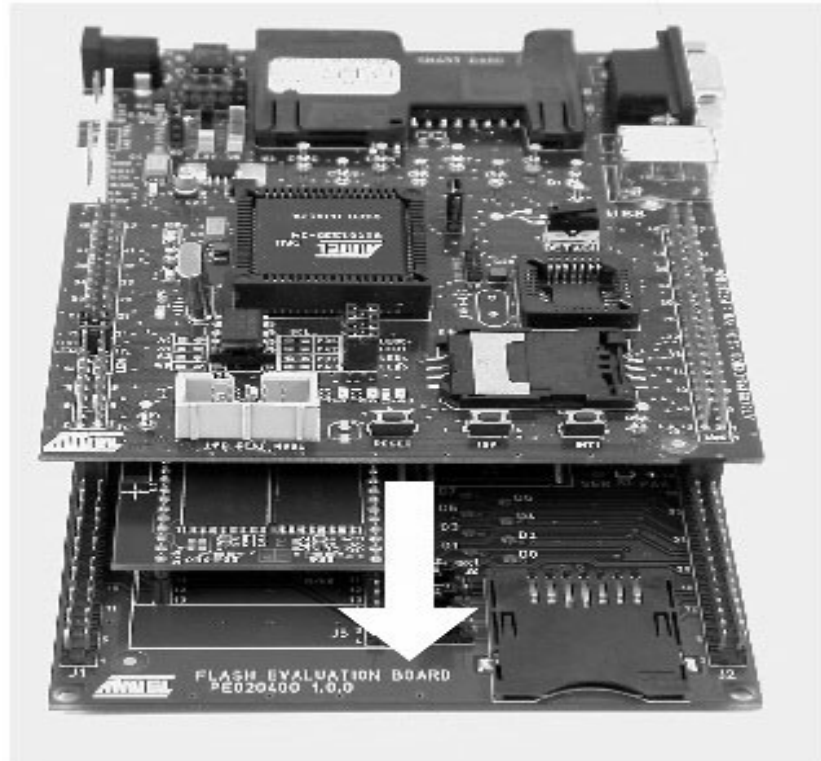
Figure 2-5. Flash evaluation board plugged to AT8xC5122D evaluation board (AT89STK03)
