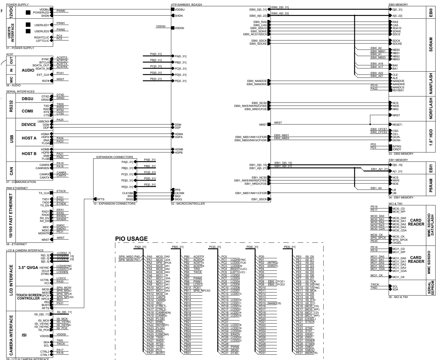
Figure 2-3. AT91SAM9263-EK Block Diagram
