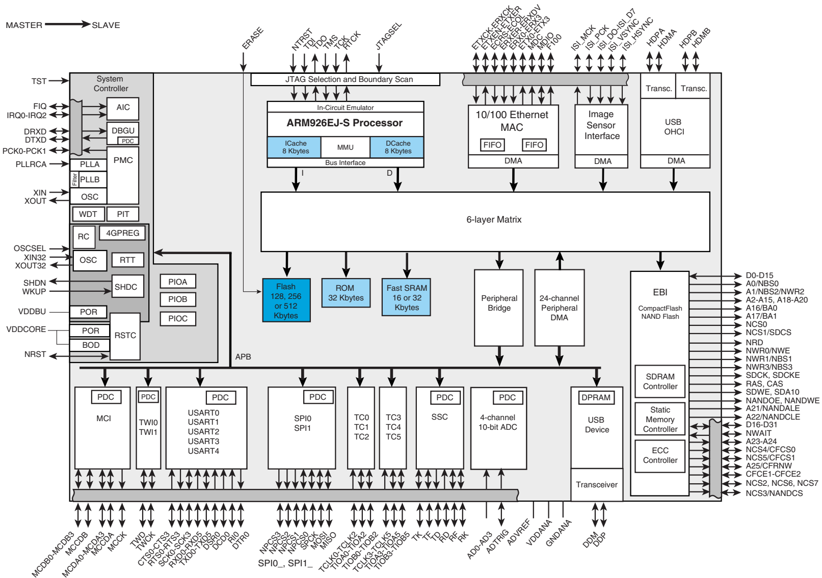
Figure 3-1. AT91SAM9XE512/256/128 Block Diagram
