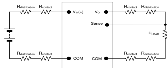
Figure 31. Remote sense circuit configuration
