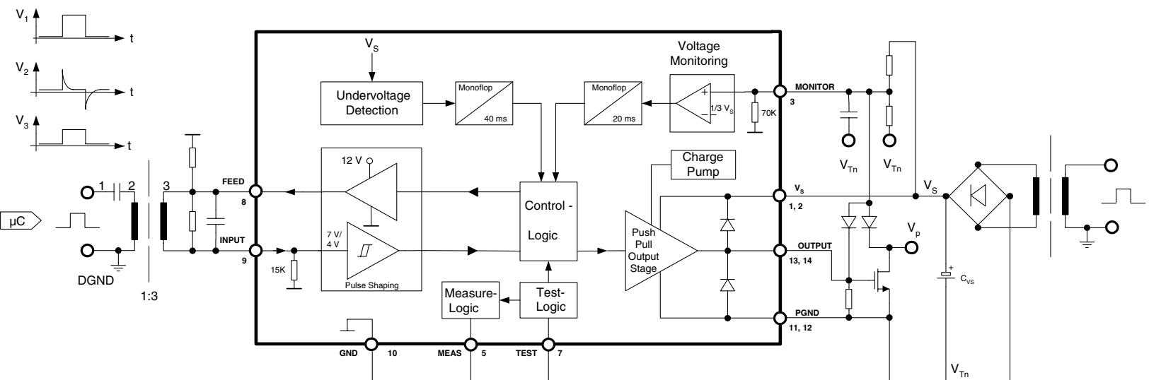
Figure 7-5. External Components for one ATA6821 in Application Circuit 3: Potential-free Control of a Three-phase Asynchronous Machine
