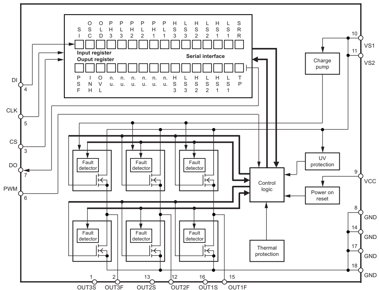
Figure 1-1. Block Diagram
