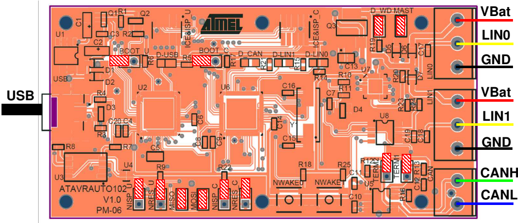
Figure 2-1. Board connections and default jumpers settings
