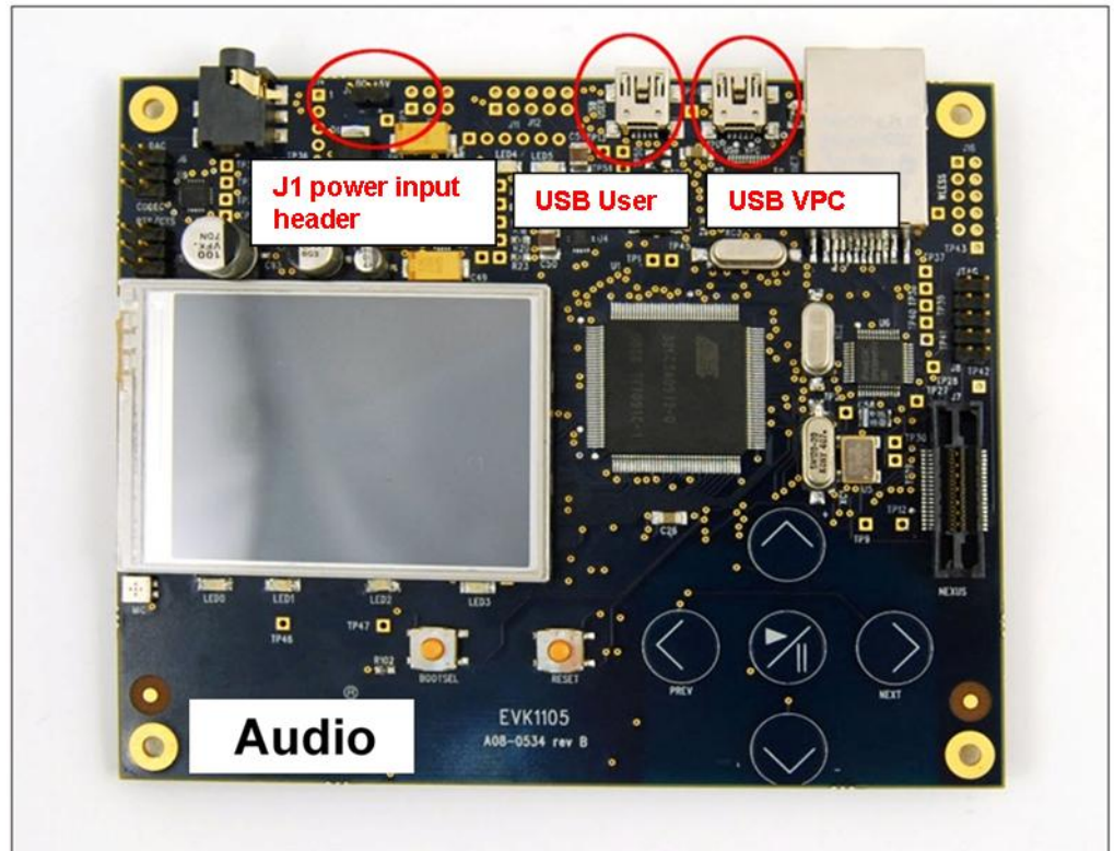
Figure 2-1 Possible power input interfaces on the EVK1105AU
