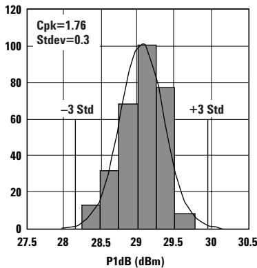
Figure 2. P1dB.
