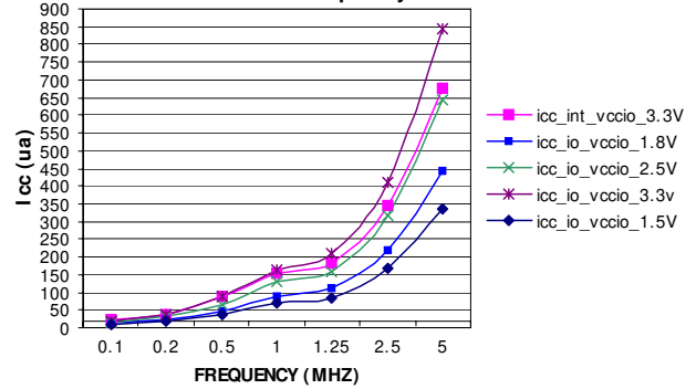
Icc_Int, Icc_io @Vccint= 1.8V (HD) over frequency
