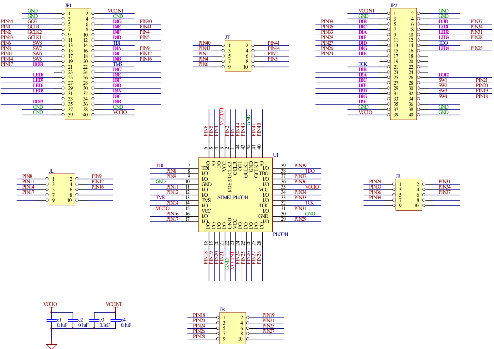
Figure 14. 44-pin PLCC Socket Adapter Board Schematic Diagram
