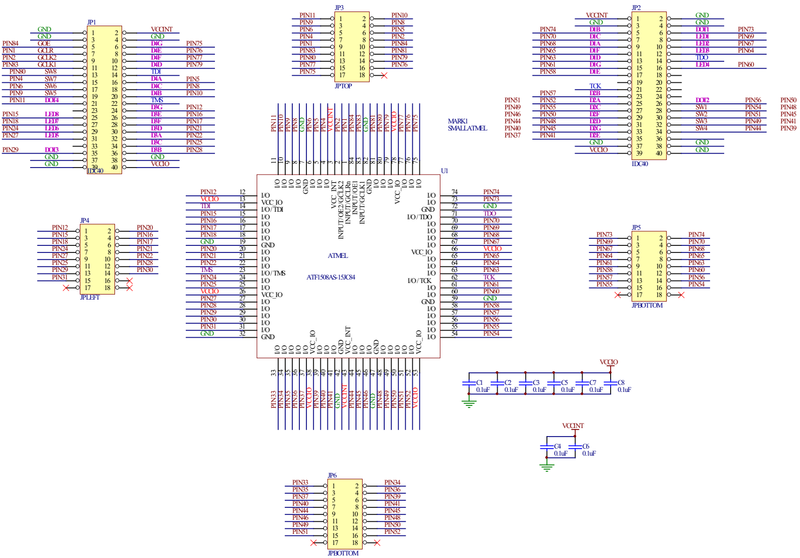
Figure 15. 84-pin PLCC Socket Adapter Board Schematic Diagram
