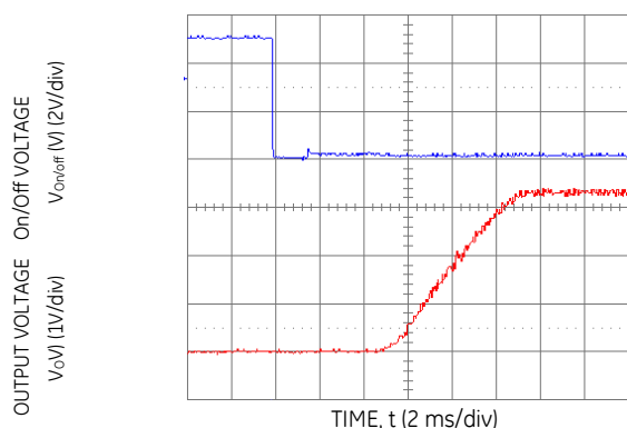
Figure 15. Typical Start-Up Using Remote On/Off with Low-ESR external capacitors ( 7 \times 150\mu\text{F} Polymer) ( V_{in} = 5.0\text{Vdc} , V_o = 3.3\text{Vdc} , I_o = 6\text{A} , C_o = 1050\mu\text{F} ).
