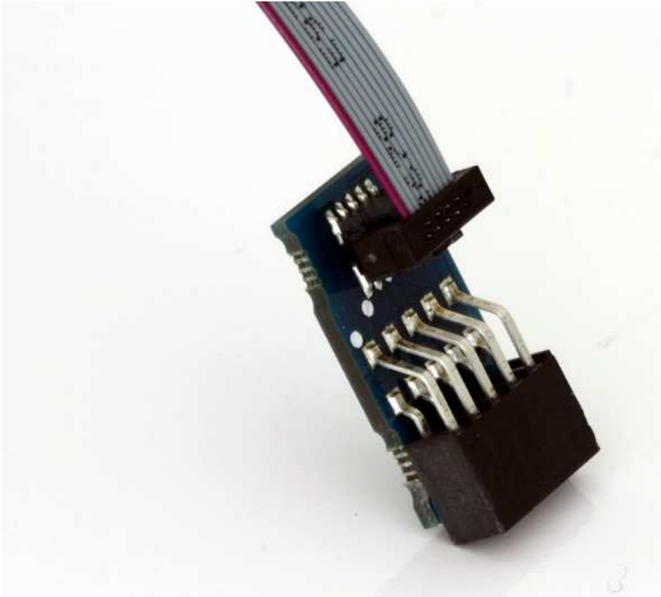
Figure 2-5. JTAGICE3 Probe Adapter Connection
