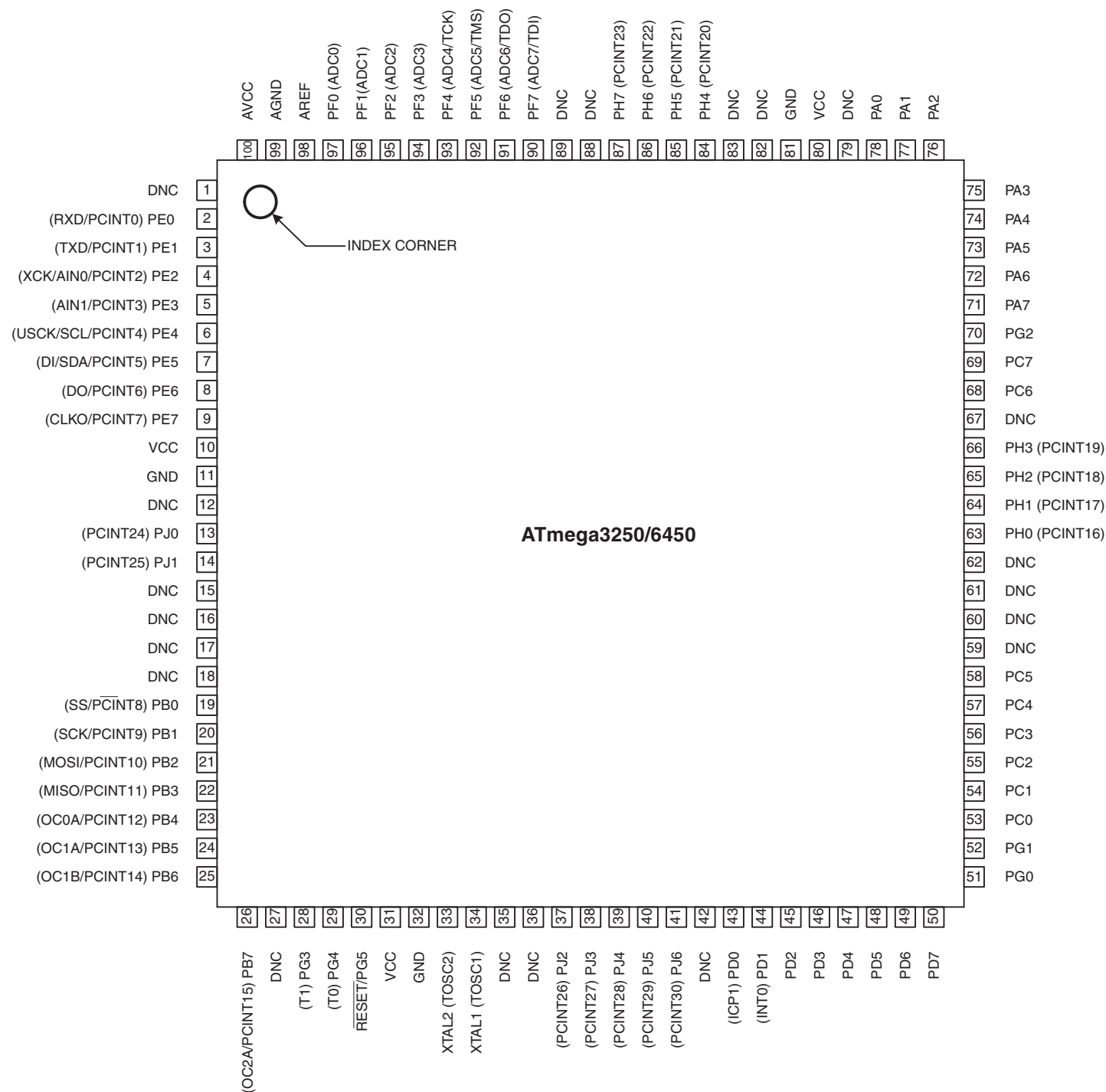
Figure 1-1. Pinout ATmega3250/6450
