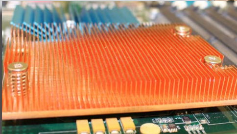
Ultra Low Profile w/ Push Pin Attachment
