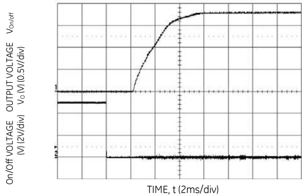
Figure 29. Typical Start-up Using Remote On/Off ( V_{IN} = V_{IN,NOM} , I_o = I_{o,max} ).
