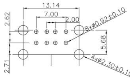
RECOMMENDED P.C.B. PATTERN LAYOUT
