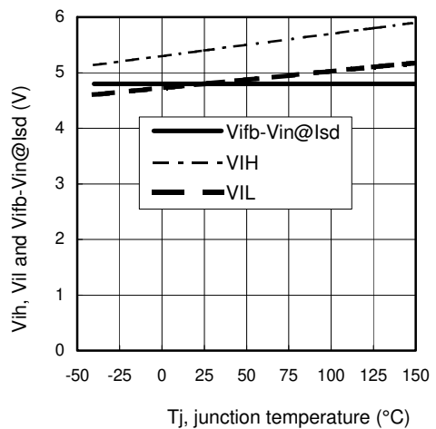
Figure 9 – V_{\text{ih}} , V_{\text{il}} and V_{\text{fb-Vin@Istd}} (V) Vs T_j ( ^\circ\text{C} )
