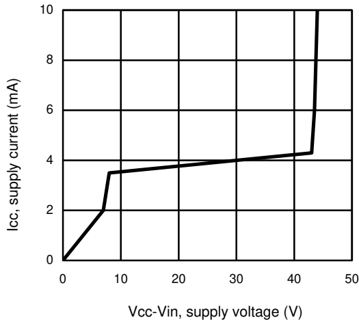
Figure 6 – I_{\text{cc}} (mA) Vs V_{\text{cc-Vin}} (V)
