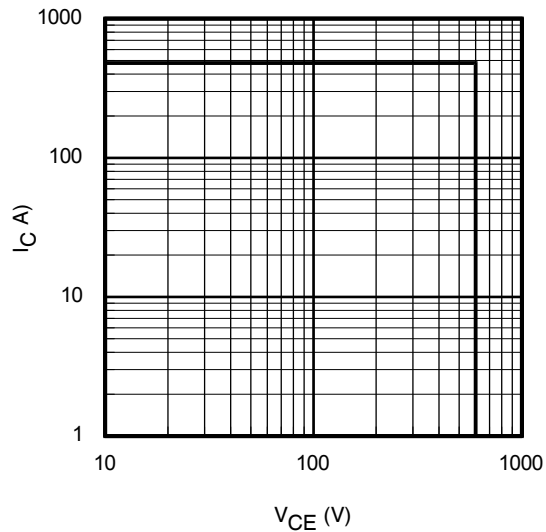
Fig. 4 - Reverse Bias SOA
