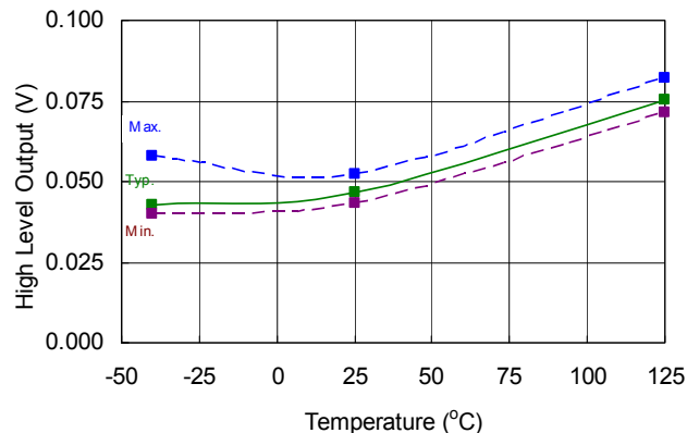
Figure 16: V_{OH} ( I_O = 2mA ) vs. temperature
