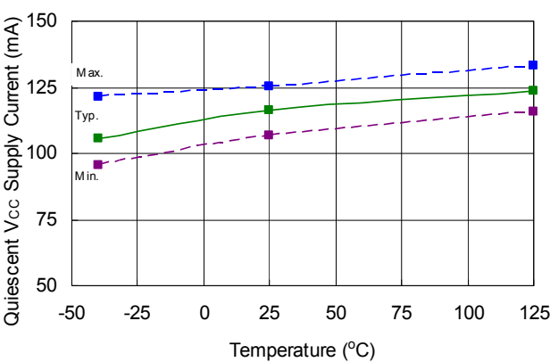
Figure 12: V CC Supply Current vs. Temperature
