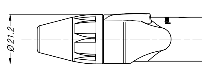
MALE CONNECTOR 1:1
