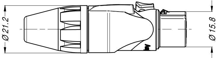
FEMALE CONNECTOR 1 : 1
