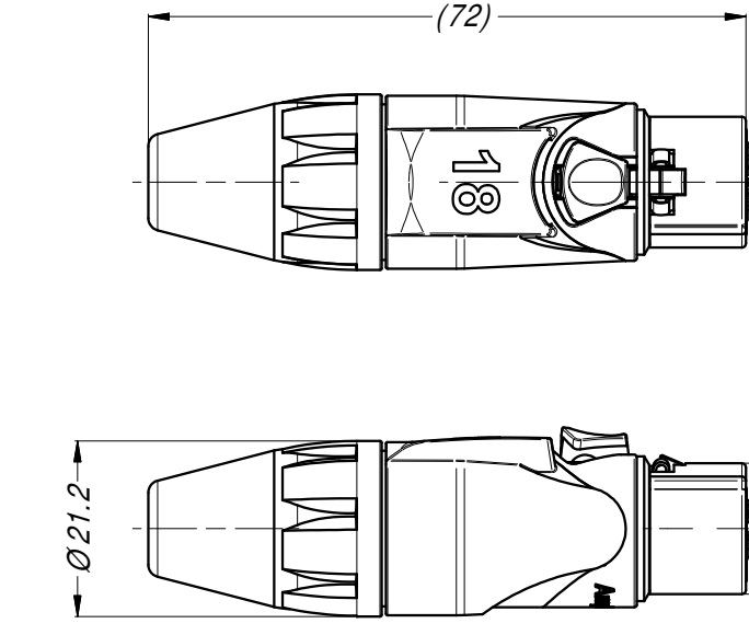
FEMALE CONNECTOR 1 : 1
