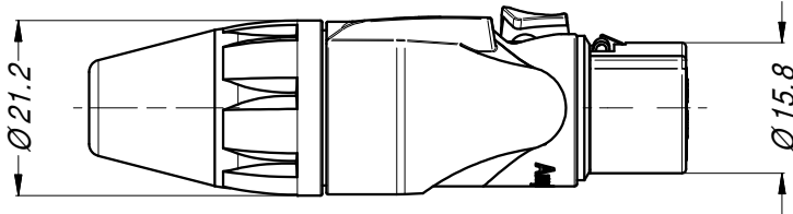
FEMALE CONNECTOR 1 : 1
