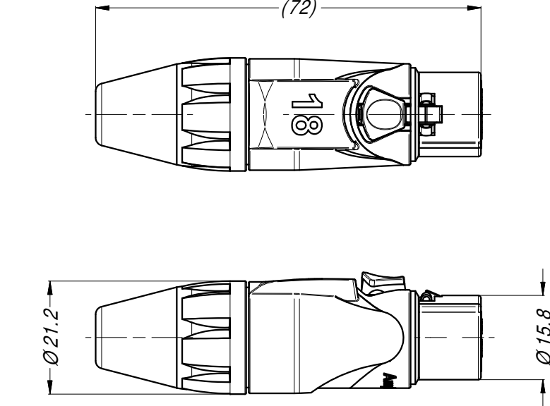
FEMALE CONNECTOR 1 : 1
