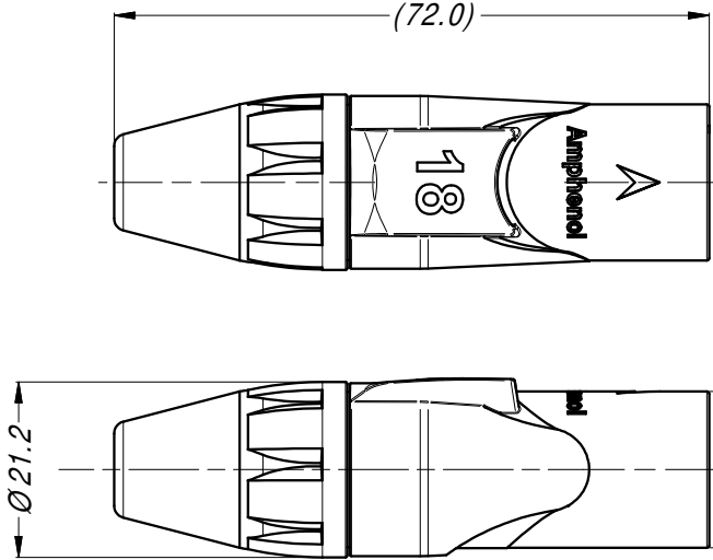
MALE CONNECTOR 1 : 1
