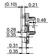
Y-Y cross section
