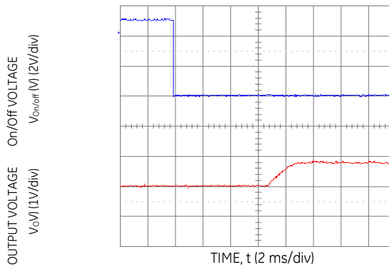
Figure 18. Typical Start-Up Using Remote On/Off with Prebias ( V_{in} = 3.3\text{ Vdc} , V_o = 1.8\text{ Vdc} , I_o = 1.0\text{ A} , V_{bias} = 1.0\text{ Vdc} ).
