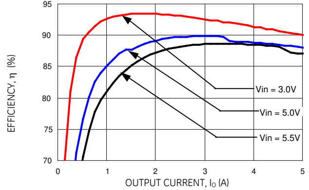
Figure 4. Converter Efficiency versus Output Current (Vout = 1.8Vdc).
