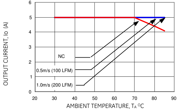
Figure 23. Derating Output Current versus Local Ambient Temperature and Airflow ( V_{in} = 3.3dc , V_o=0.75 Vdc ).
