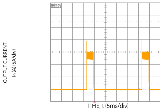
Figure 19. Output short circuit Current ( V_{in} = 5.0\text{ Vdc} , V_o = 0.75\text{ Vdc} ).
