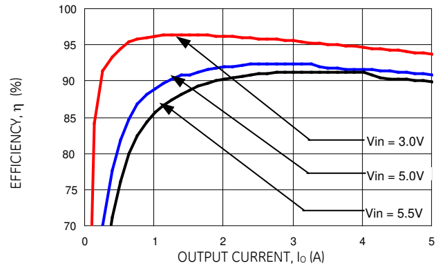
Figure 5. Converter Efficiency versus Output Current (Vout = 2.5Vdc).
