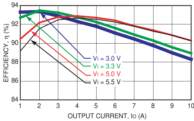
Figure 7. Converter Efficiency vs Output Current AXH010A0Y (1.8V Output Voltage).
