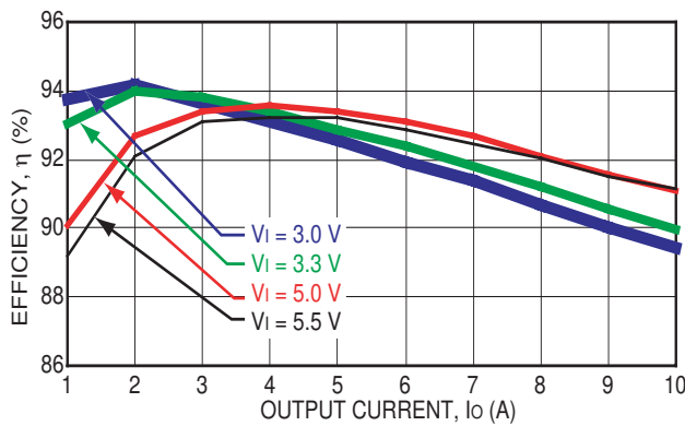
Figure 8. Converter Efficiency vs Output Current AXH010A0D (2.0V Output Voltage).
