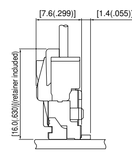
PA Receptacle + PA Header (Retainer mountable type)
