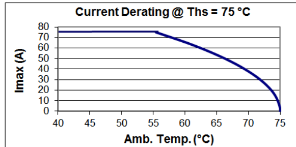
B25620B1287K103
