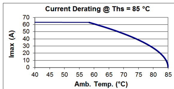
B25620B1427A101
