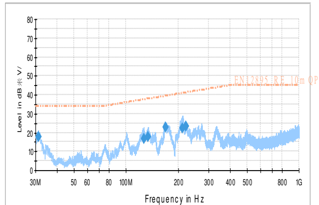
Figure 19: test result(Horizontal)
