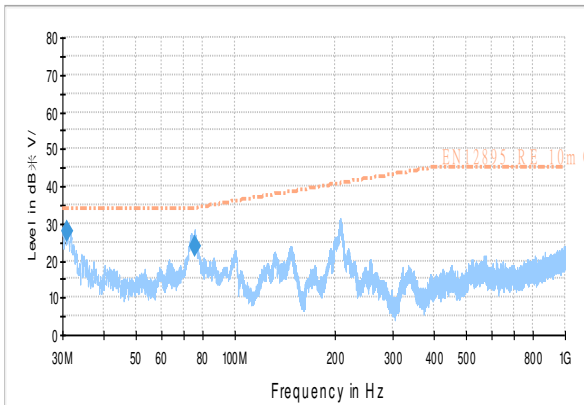
Figure 18: test result(Vertical)
