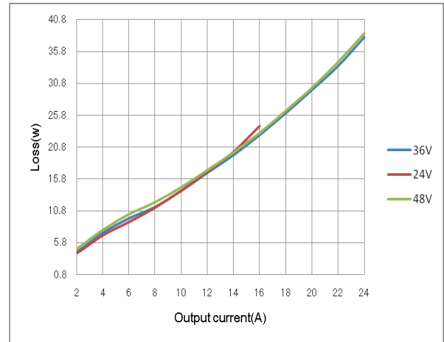
Figure 2: Loss vs. Output current @ Vin=24V,36V,48V (for A/B/C/D/H)
