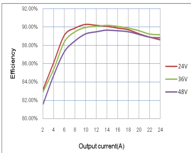
Figure 1: Efficiency vs. Output current Vin=24V,36V,48V (for A/B/C/D/H)
