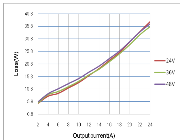
Figure 2: Loss vs. Output current @ Vin=24V,36V,48V (for A/B/C/D/H)
