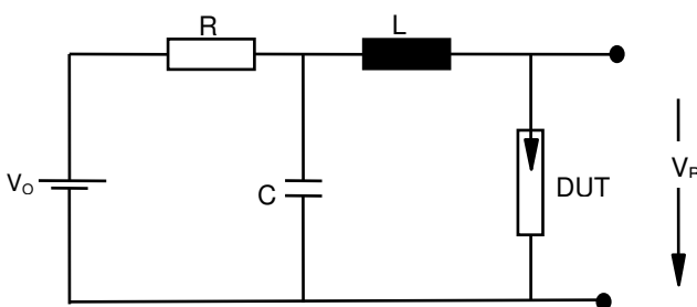
Fig. 3: QC- test circuit (sampling inspection at 25
