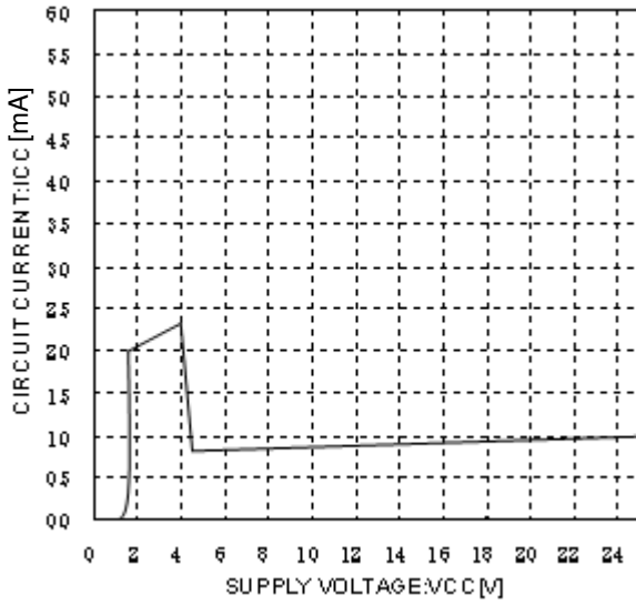
Fig.13 Circuit Current
