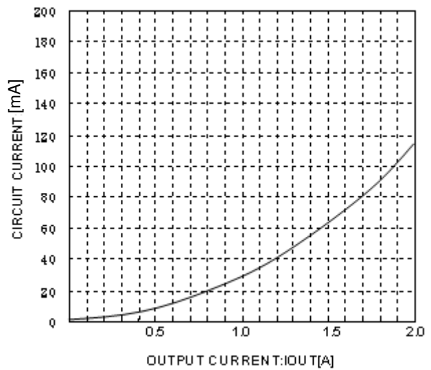
Fig.20 Circuit Current by load Level (I OUT =0mA→2A)
