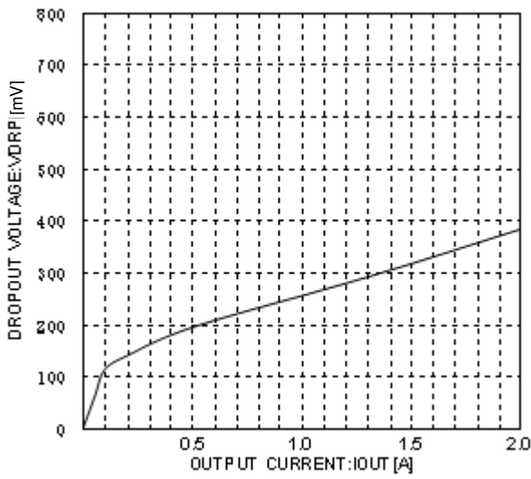
Fig.17 Input/Output Voltage Difference I out -ΔV d Characteristics (V cc =4.75V)
