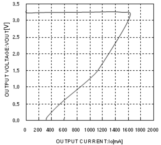
Fig.4 Load Stability
