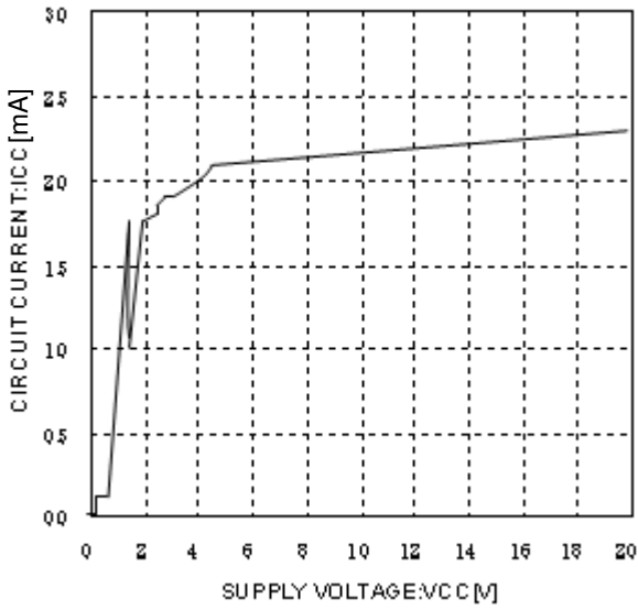
Fig.1 Circuit Current
