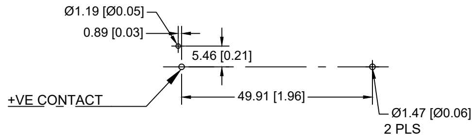
PCB LAYOUT
