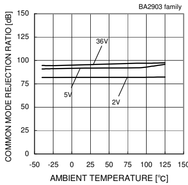
Fig.80 Common Mode Rejection Ratio - Ambient Temperature
