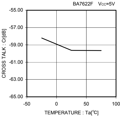
Fig.55 Cross talk vs. Temperature
