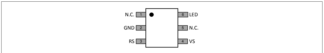
Figure 2 Pinout BCR430
