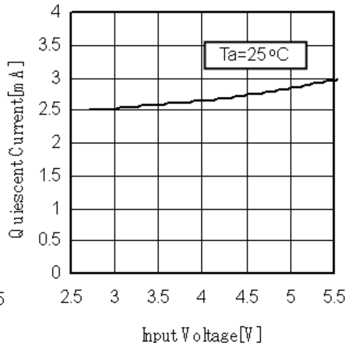
Figure 3. Quiescent Current2
