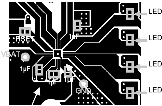
Wiring from the VBAT pin to Cin must meet a low impedance.
