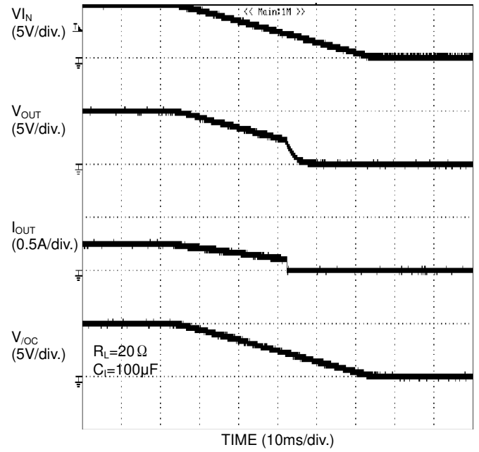
Figure 35. UVLO response Decreasing V_{IN} (BD2045AFJ)
