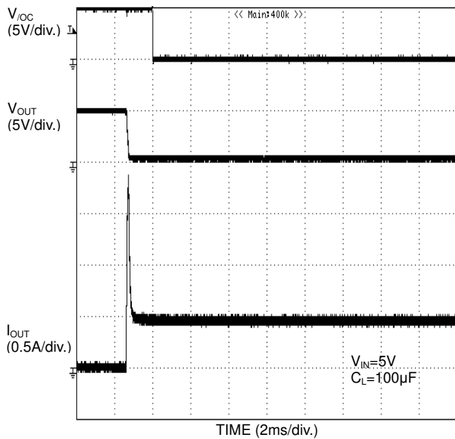
Figure 32. Over current response Enabled to short-circuit (BD2045AFJ)
