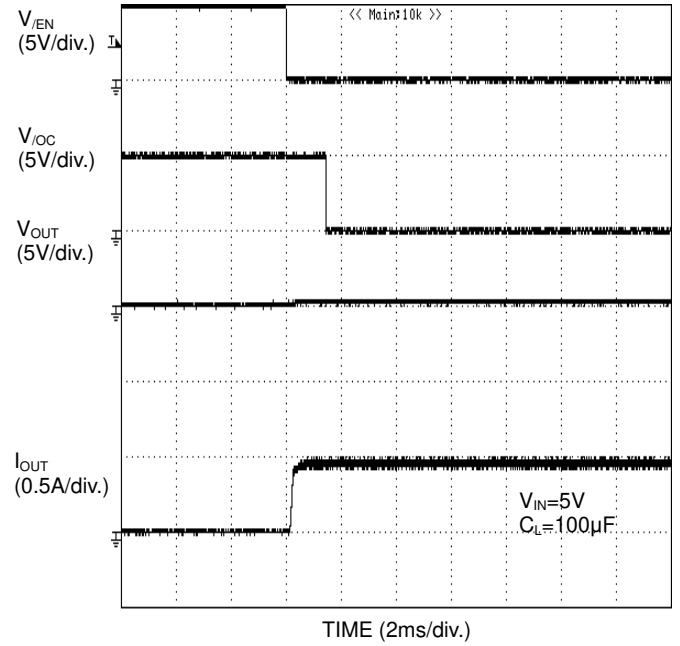
Figure 31. Over current response Enabled to short-circuit (BD2045AFJ)
