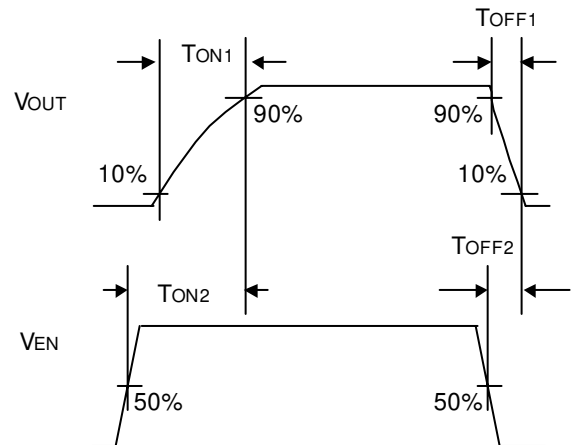
Figure 3. Timing diagram (BD2055AFJ)
