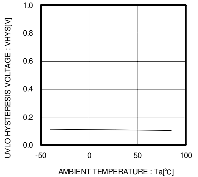
Figure 25. UVLO hysteresis voltage
