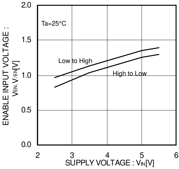
Figure 8. EN L /EN H input voltage
