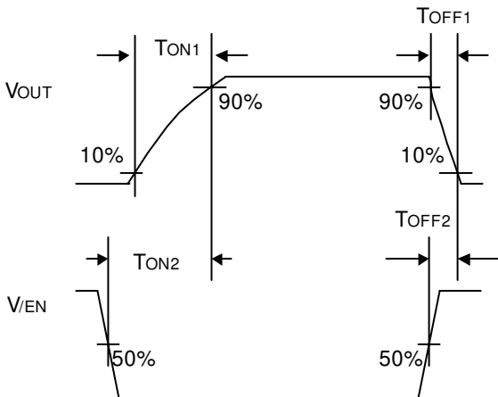
Figure 2. Timing diagram (BD2045AFJ)
