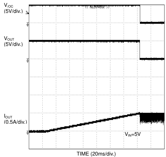
Figure 29. Over current response Ramped load (BD2045AFJ)
