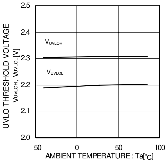
Figure 24. UVLO threshold voltage
