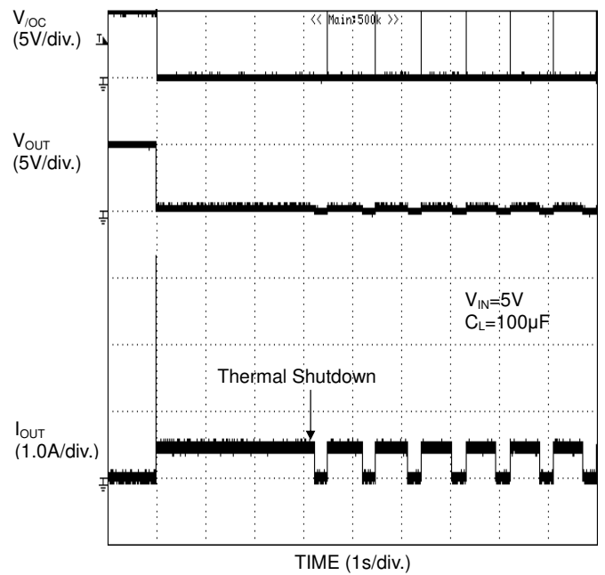
Figure 33. Over current response Enabled to short-circuit (BD2045AFJ)
