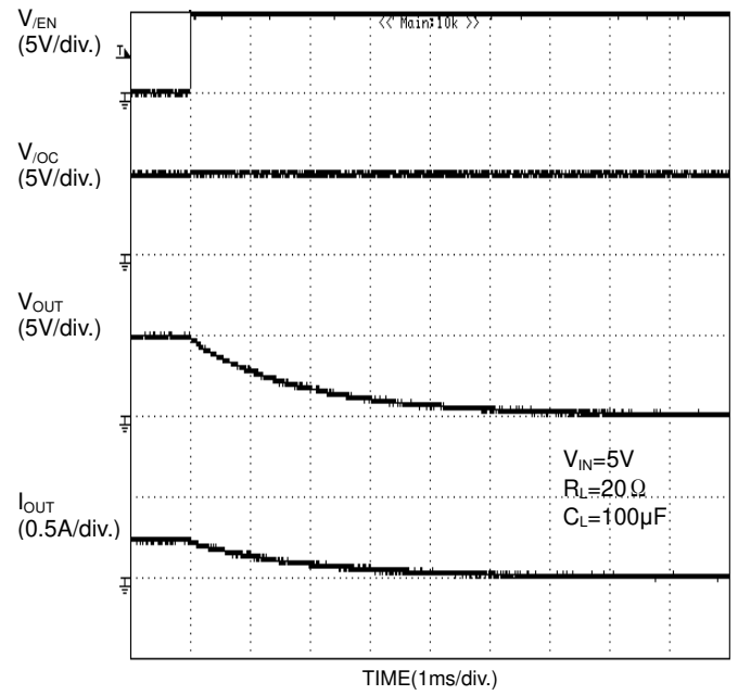
Figure 27. Output fall characteristic (BD2045AFJ)
