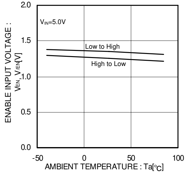
Figure 9. EN L /EN H input voltage
