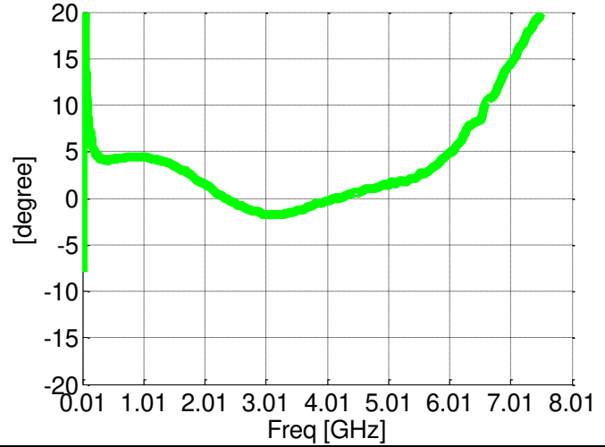
Phase balance
