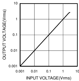
Fig.7 Output Voltage - Input Voltage
