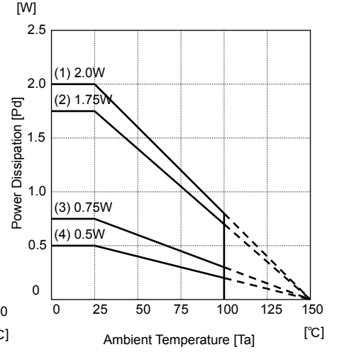
◎HQFN20V(BD3533EKN)
